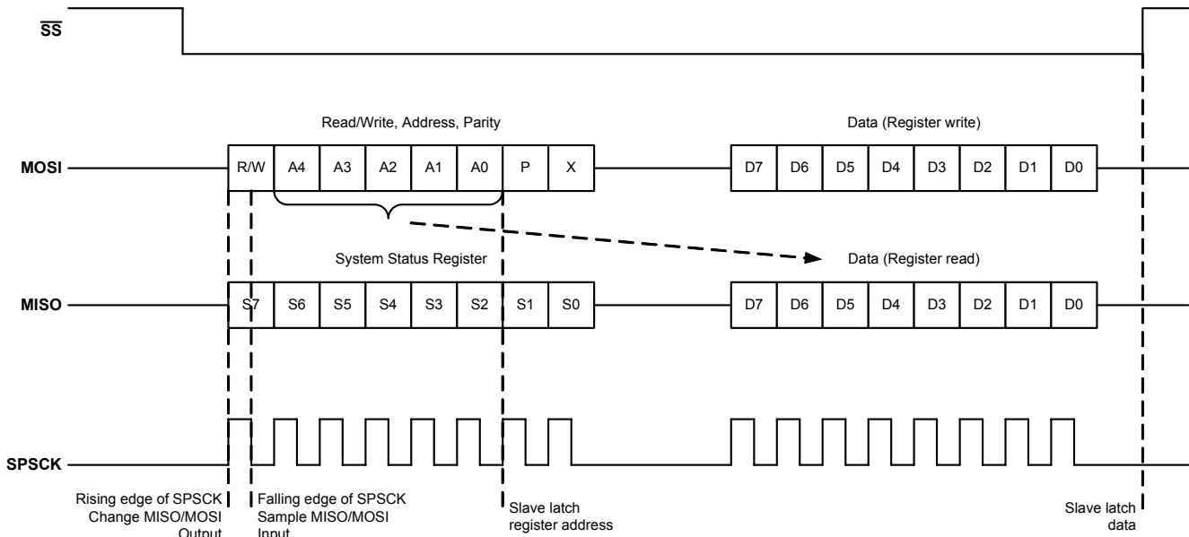
Figure 11. SPI Protocol
