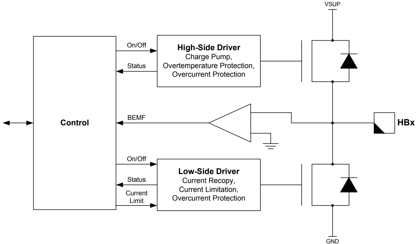
Figure 12. Half-bridge Push-Pull Output Driver
